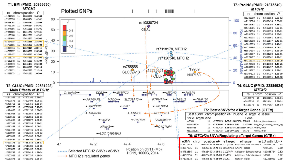
Figure 4. Selected SNVs of MTCH2 Significantly Associating with BMI, Glucose, Insulin, and a Few of Them Regulating the Expression (eSNVs) of at Least Four Genes: C1QTNF4, SLC39A13, PSMC3, and CELF1
